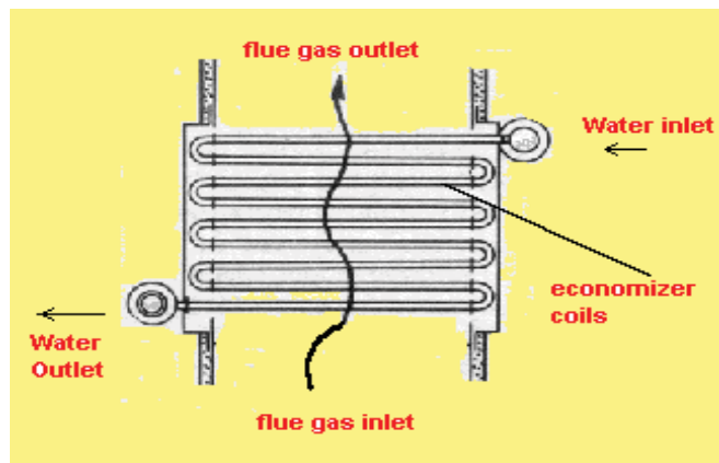
Figure 8.8 Economiser
