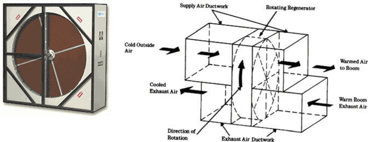
Figure 8.6 Heat Wheel
