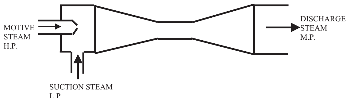
Figure 8.13 Thermocompressor
