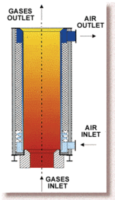
Figure 8.2 Metallic Radiation Recuperator
