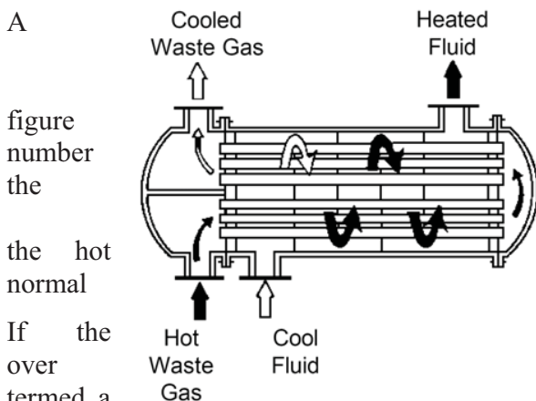
Figure 8.3 Convective Recuperator
