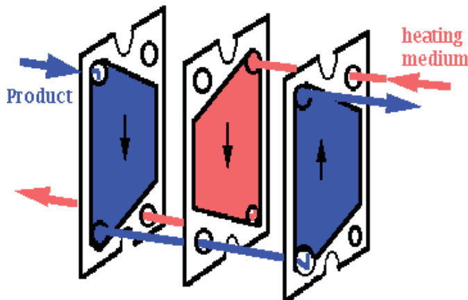
Figure 8.10 Plate Heat Exchanger
