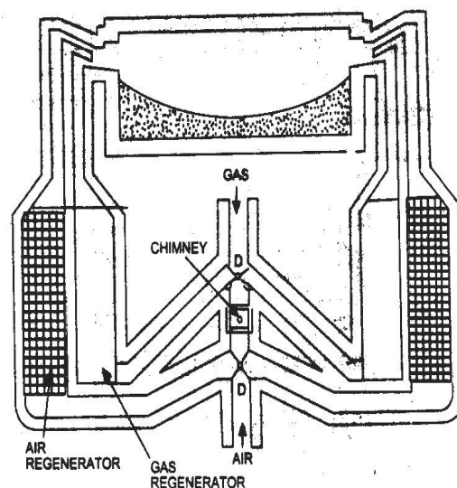
Figure 8.5 Regenerator
