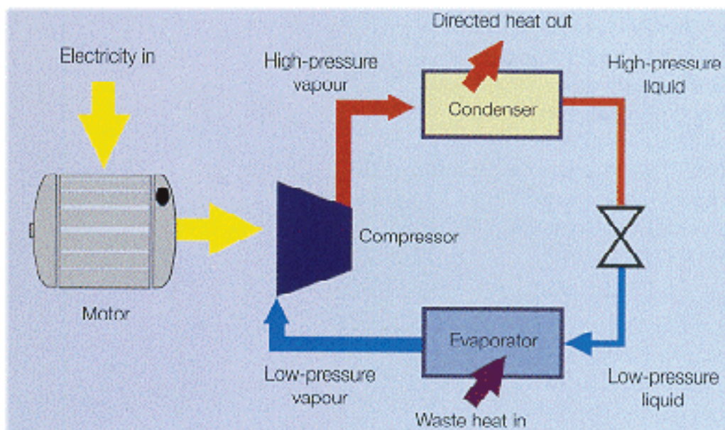
Figure 8.12 Heat pump
