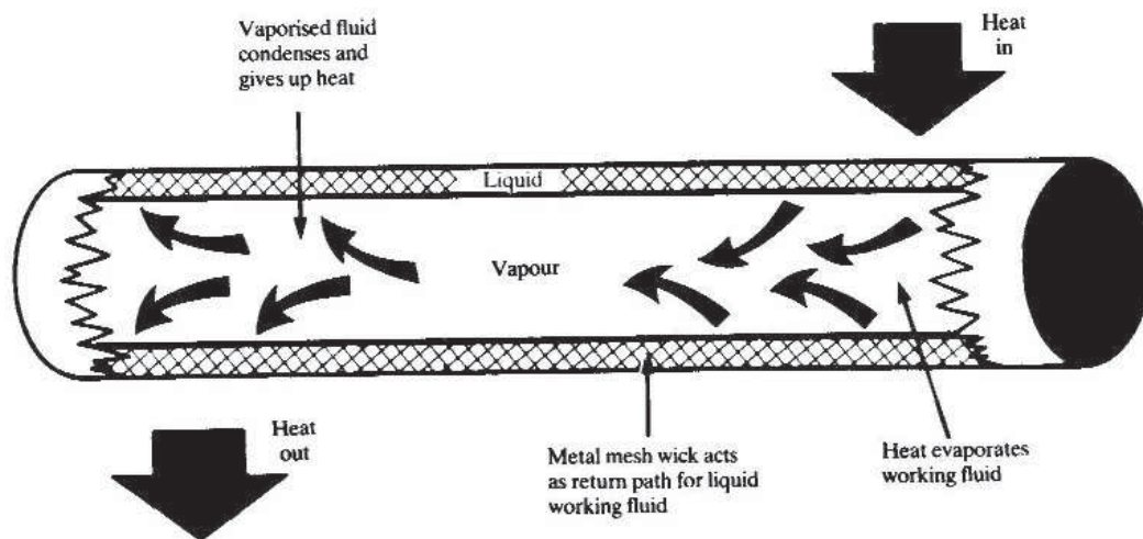
Figure 8.7 Heat Pipe
