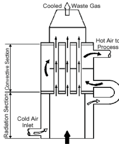
Figure 8.4 Convective Radiative Recuperator
